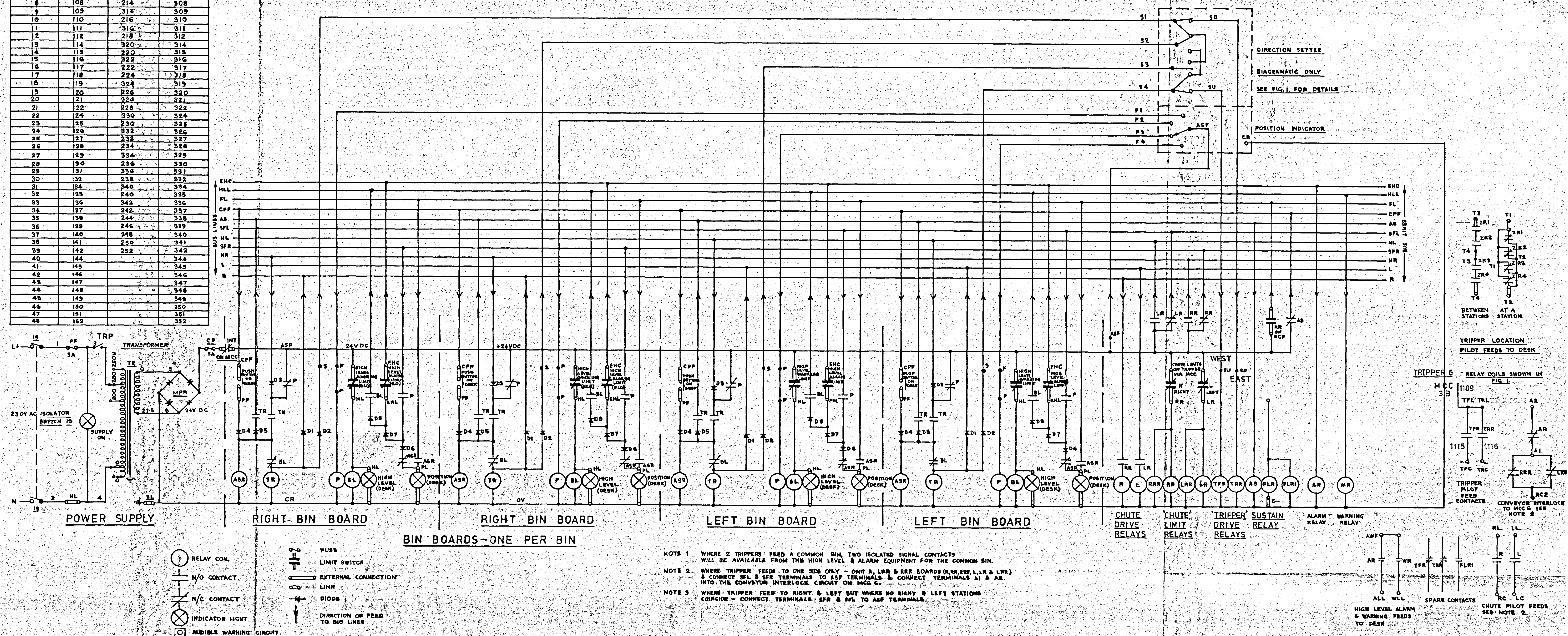
FIG. 1. SELECTOR FOR POSITION & DIRECTION
